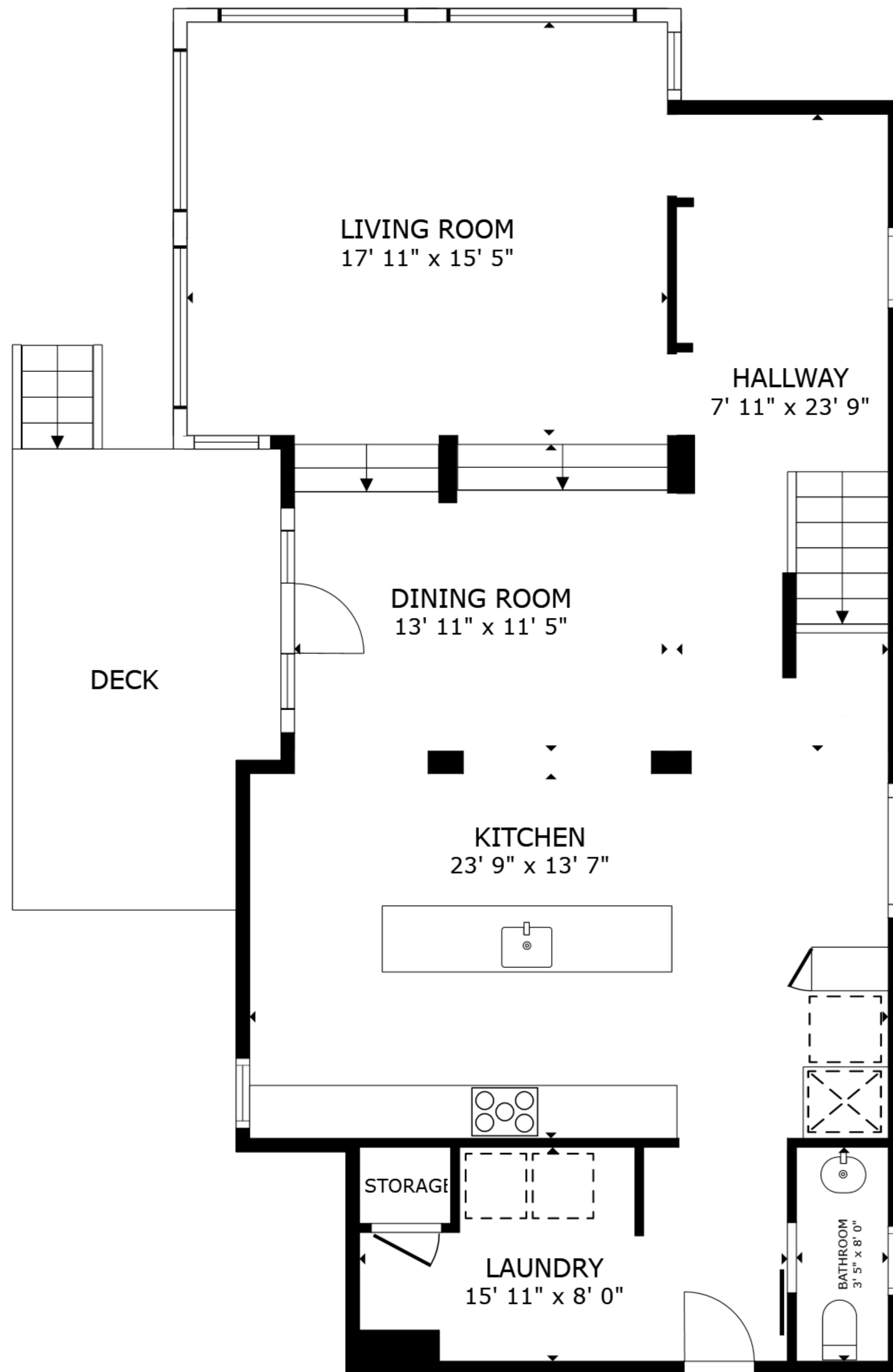
FLOOR 1
